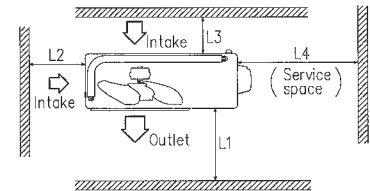
Minimum installation space
